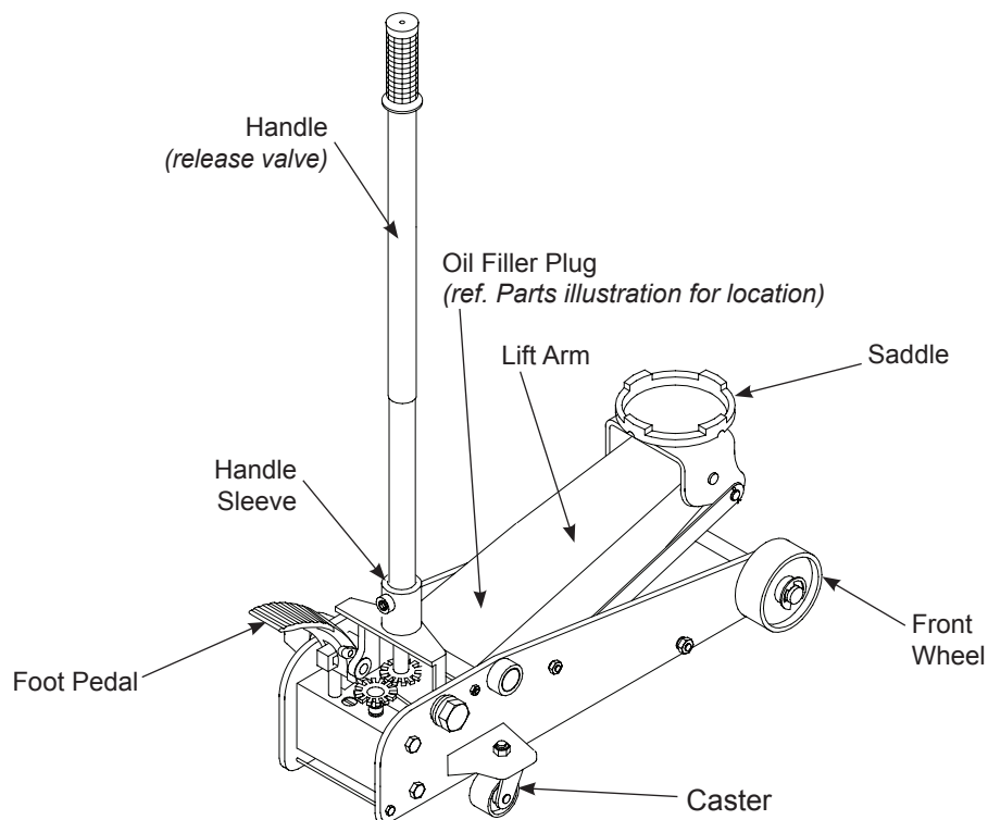
Figure 1 - Typical Jack Nomenclature
