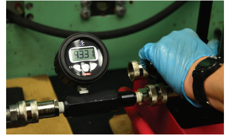
GE2514 Back-Lit digital pressure gauge displays in: PSI, BAR, KG/CM2 and MPa
